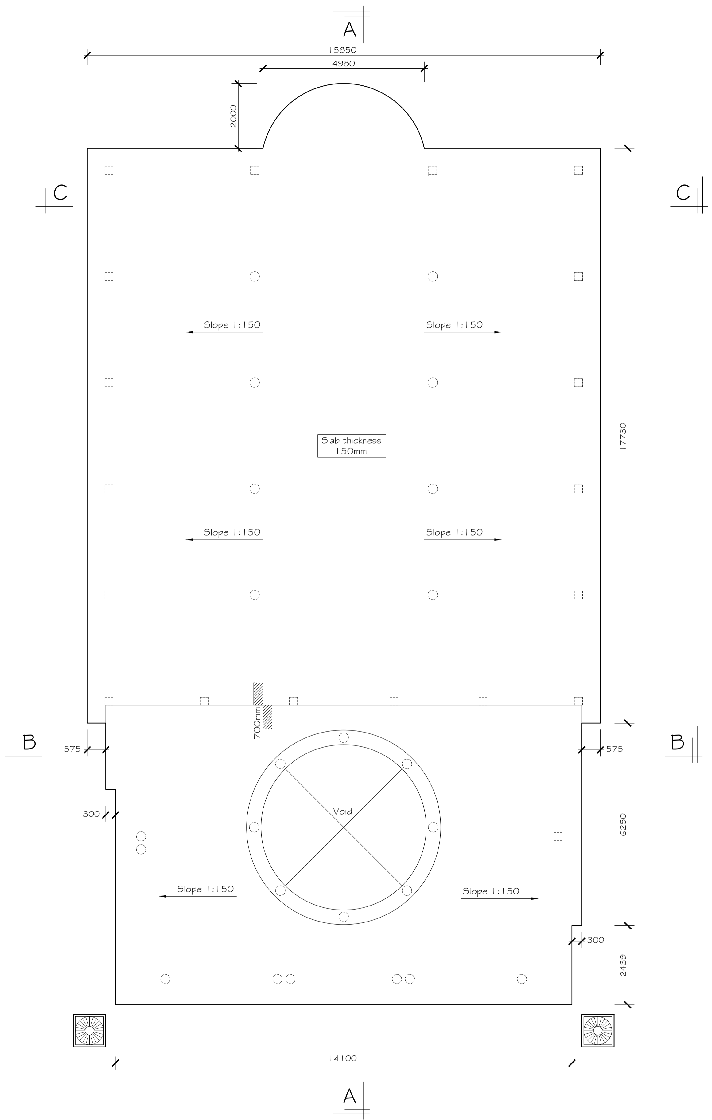
ROOF PLAN
